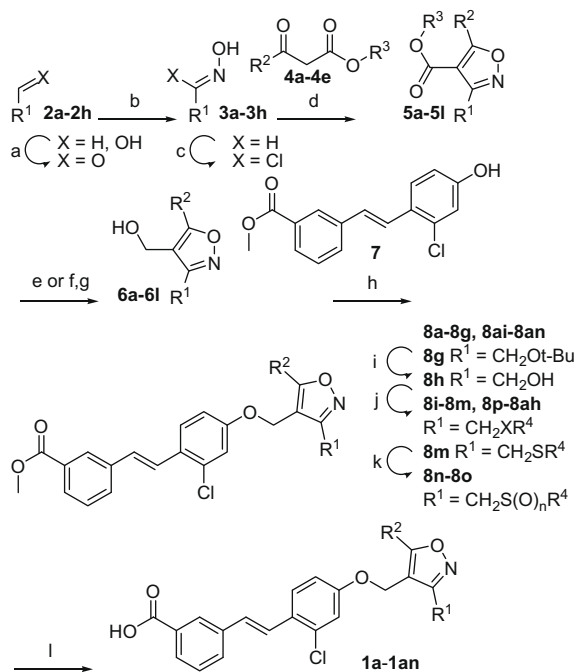
Scheme 1. Reagents and conditions: (a) SO 3 -pyridine, DMSO, NEt 3 , CH 2 Cl 2 , 0 °C–rt; (b) NH 2 OH·HCl, NaOH, EtOH, H 2 O, 31–88% for 2 steps; (c) NCS, DMF; (d) 4a–e , NaOMe, THF, 21–63% for 2 steps; (e) i Bu 2 AlH, THF, 0 °C–rt, 14–99%; (f) 6b , NaOH, H 2 O, MeOH, THF, microwave@100 °C, 81%; (g) i PrO(C=O)Cl, THF, NEt 3 ; NaBH 4 , H 2 O, 59%; (h) 7 , DIAD, PPh 3 , toluene, microwave@80 °C, 21–76%; (i) TFA, CH 2 Cl 2 , 78%; (j) DIAD, PPh 3 , phenols 9a–b and 9f–w , trifluoroacetamides 9c–d , thiophenol 9e , or thiotetrazole 9x , toluene, microwave@80 °C, 22–73%; (k) m -CPBA, CH 2 Cl 2 , 0 °C–rt, 40% and 40%, respectively; (l) NaOH, MeOH, THF, H 2 O, microwave@100 °C, 42–99%.
